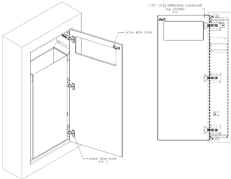
BREAKOUT VIEW FWO/CABINET INTERIOR
