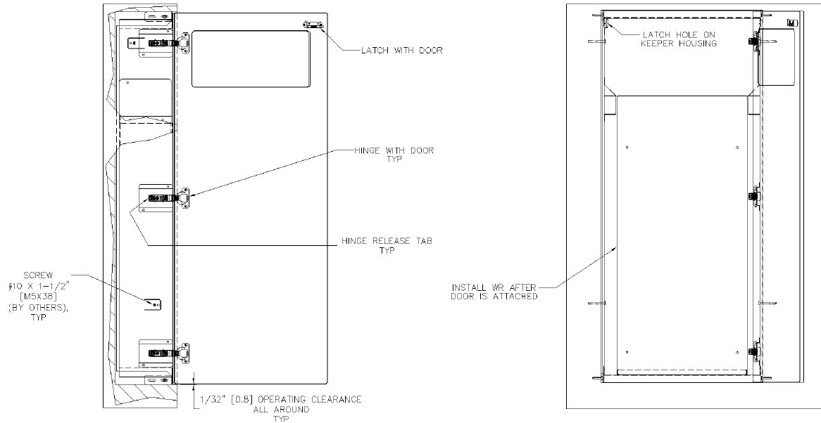
BREAKOUT VIEW FWO/CABINET INTERIOR
