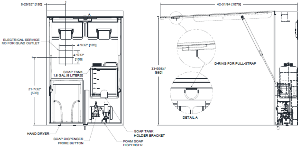
OPEN VIEW (-1, -2)
