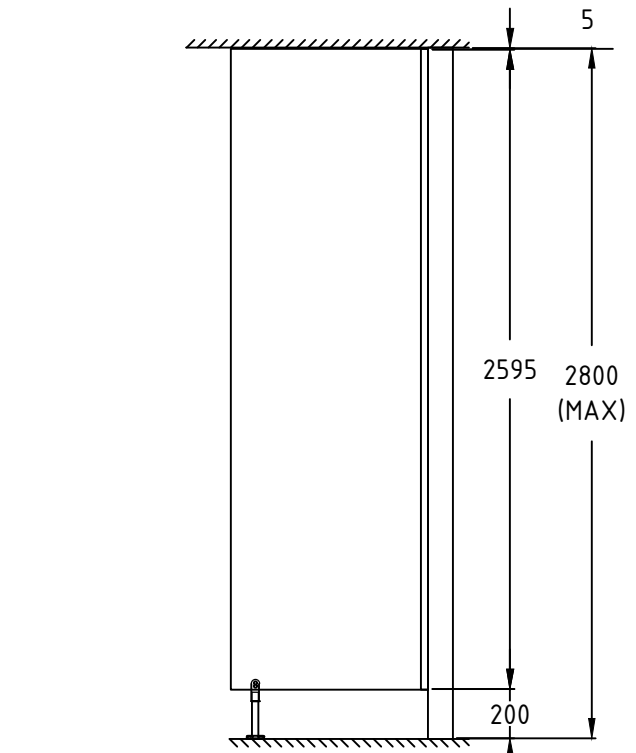
URINAL SCREEN SIDE ELEVATION
