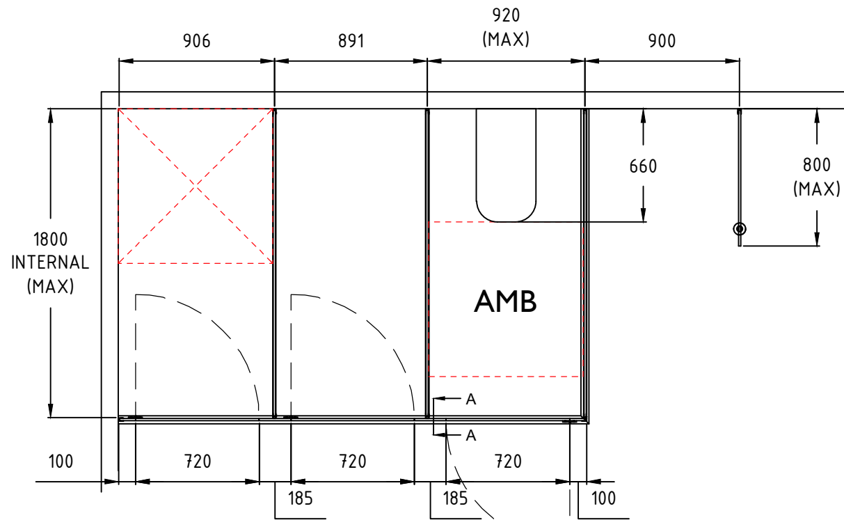
PARTITION LAYOUT
