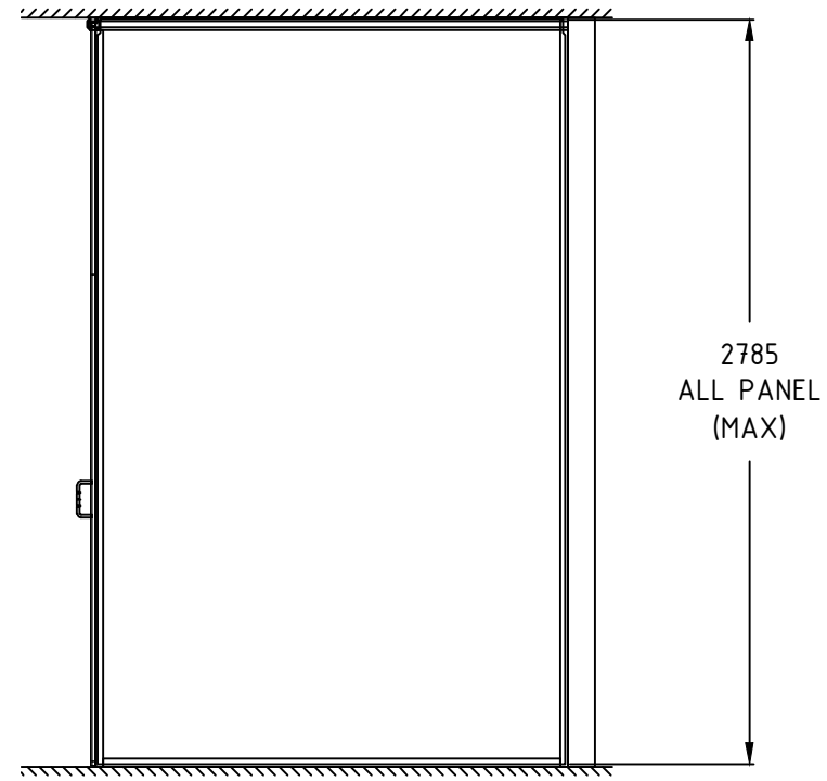
PARTITION SIDE ELEVATION
