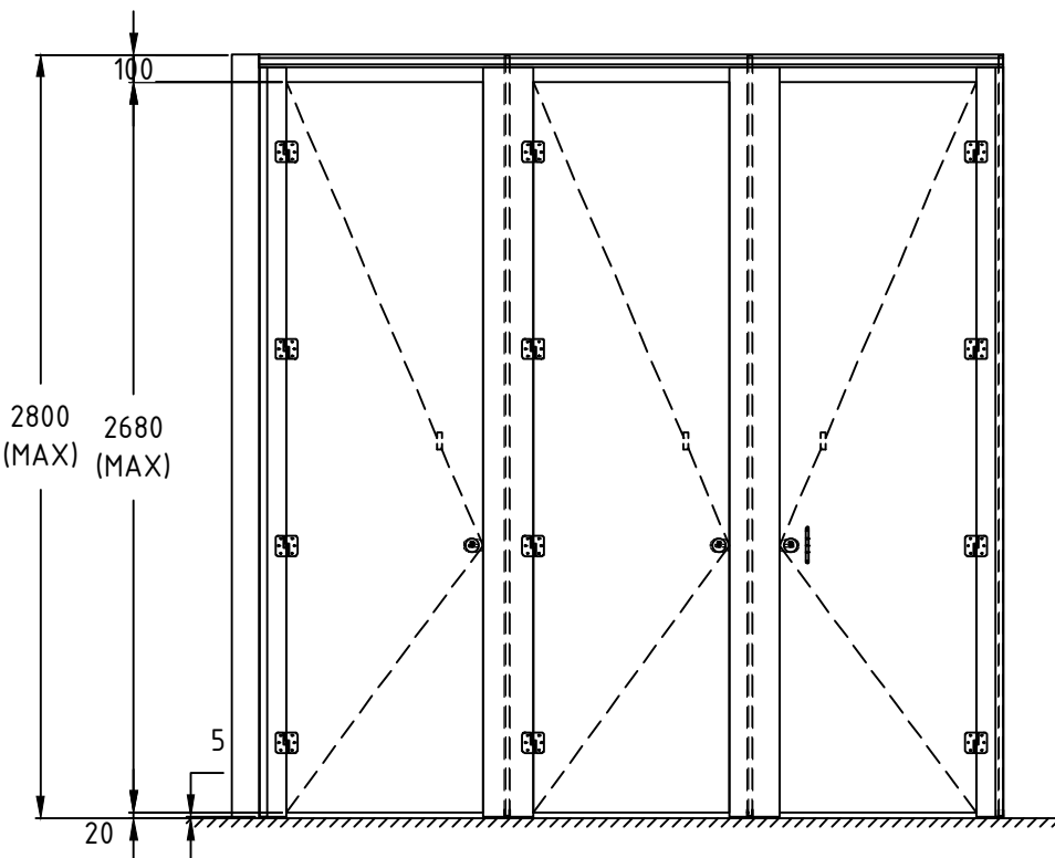
PARTITION FRONT ELEVATION OPTION 1
