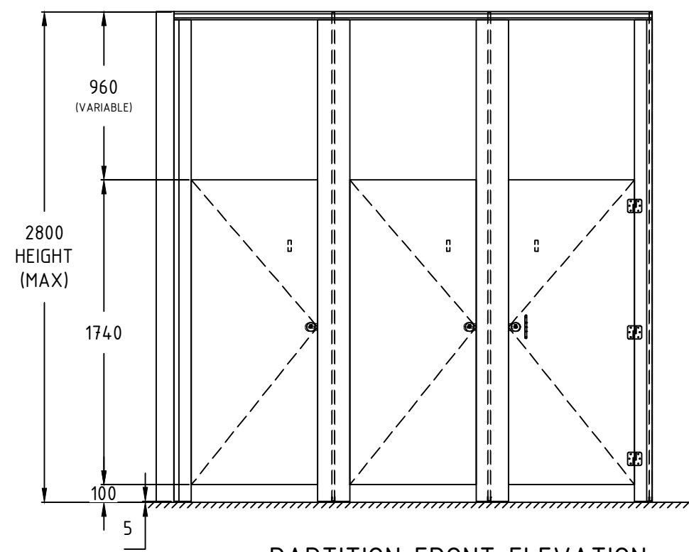
PARTITION FRONT ELEVATION OPTION 2
